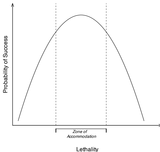
Figure 1.: H1 Visualization
